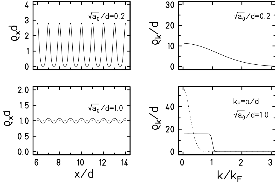
FIG. 6. Upper part: section of spatial density of hundred gaussians (not overlapping in coordinate space) and corresponding momentum distribution (same for all). Antisymmetrization does not change the distribution. Lower part: same as above but for overlapping gaussians. Full line with antisymmetrization, dash-dotted line without. For details see text.
