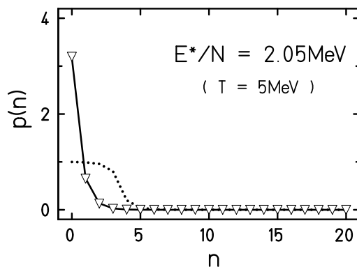
FIG. 11. Occupation numbers for a product state (Boltzmann statistics). Ergodic ensemble (triangles), canonical ensemble (solid line), both for an excitation energy of E^*/N = 2.05 MeV which corresponds to a temperature T = 5 MeV in the canonical ensemble. The dotted line shows the result for Fermi-Dirac statistics at the same temperature.
