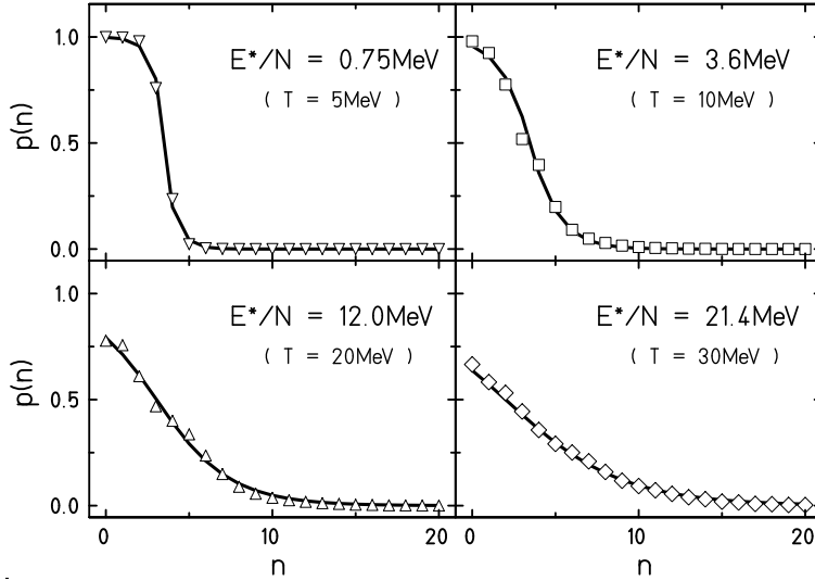
FIG. 9. Occupation numbers calculated in the ergodic ensemble \overline{\langle \tilde{c}_n^+ \tilde{c}_n \rangle}_{|\langle \tilde{H} \rangle} (symbols) compared with the canonical ensemble \langle \langle \tilde{c}_n^+ \tilde{c}_n \rangle \rangle_T (solid line).
