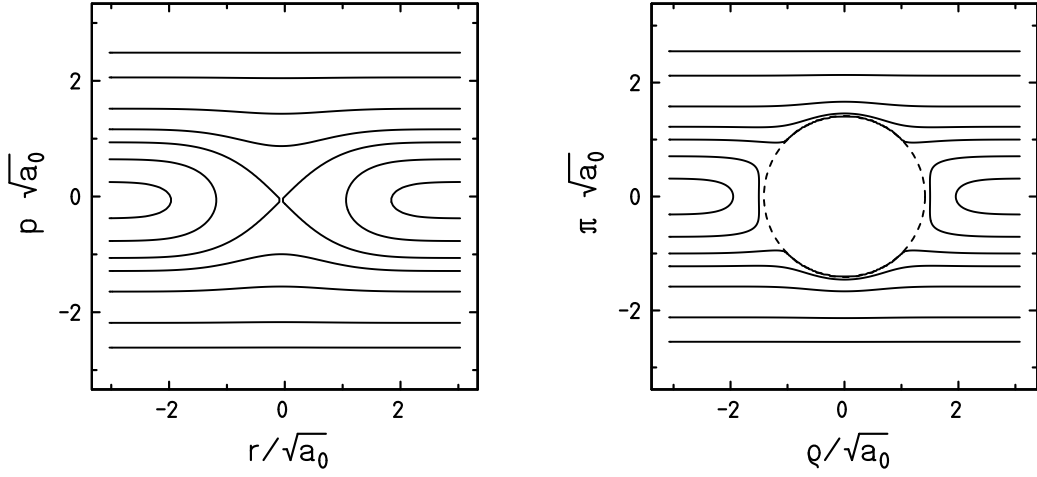
FIG. 4. Trajectories in phase space of one-dimensional free motion with fixed width.
