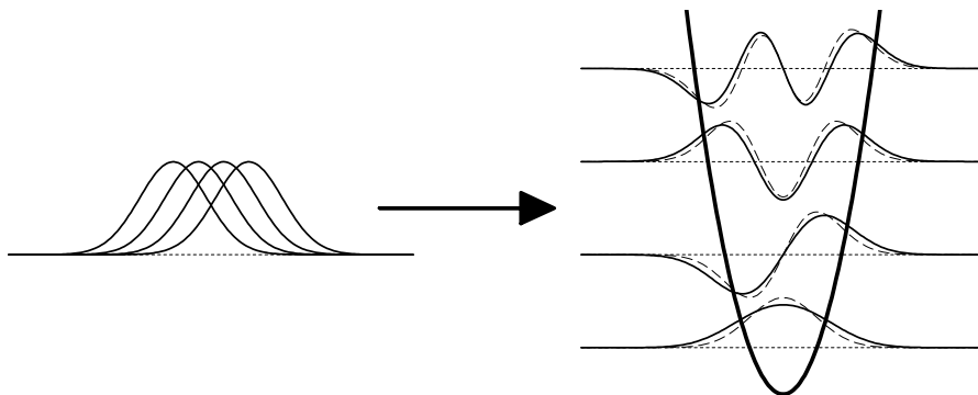
FIG. 5. Antisymmetrization of the four gaussians (l.h.s.) leads to harmonic oscillator states (r.h.s.). Dashed lines are the exact eigenstates of the oscillator.
