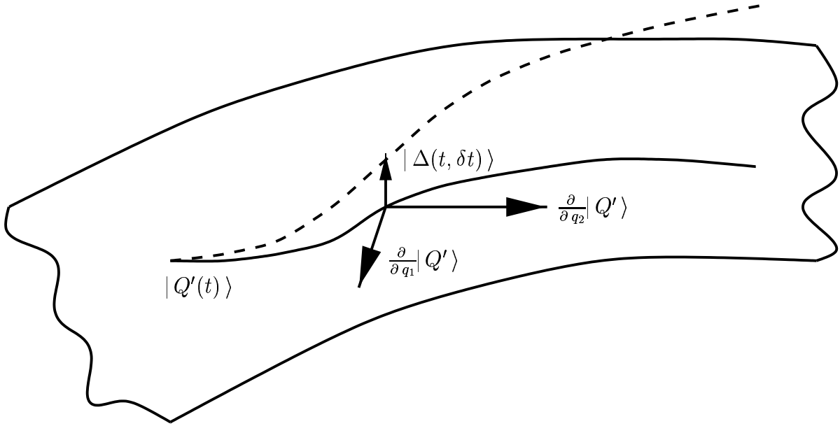
FIG. 1. Sketch of the manifold of trial states with the approximate time evolution (solid line) and the solution of the Schrödinger equation (dashed line). The error |\Delta(t, \delta t)\rangle is orthogonal to all tangent states \frac{\partial}{\partial q_\nu}|Q'\rangle .
