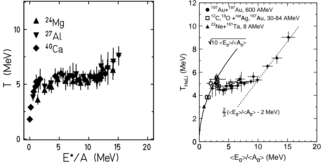
FIG. 12. L.h.s.: caloric curve of ^{24}\text{Mg} , ^{27}\text{Al} and ^{40}\text{Ca} at \hbar\omega = 1 MeV, r.h.s.: caloric curve determined by the Aladin group from the decay of spectator nuclei.
