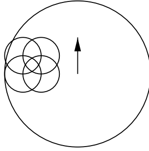
FIG. 2. Sketch of a four particle cluster and a passing wave packet. Circles indicate half-density contours. The equations of motion for the centroids and the widths of the packets can only influence the passing wave packet as a whole (see text).
