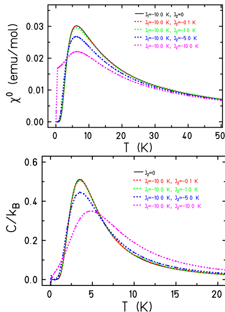
FIG. 3. (Color online) Zero-field susceptibility and specific heat of the one-dimensional spin system shown in Fig. 1 (a) for various interdimer couplings J_2 and B = 0 . Fluctuations of C at the lowest T result from very slow and thus insufficient convergence.
