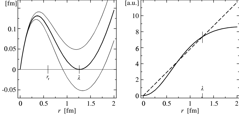
Fig. 3. L.h.s.: Coordinate transformation R_-(r) plotted as r - R_-(r) for E = 0 and different N_0 . R.h.s.: Exact radial wave function u_{E=0}(r) (solid line) and trial function u(r) for which R_-(\lambda) = \lambda and R'_-(\lambda) = 1 .
