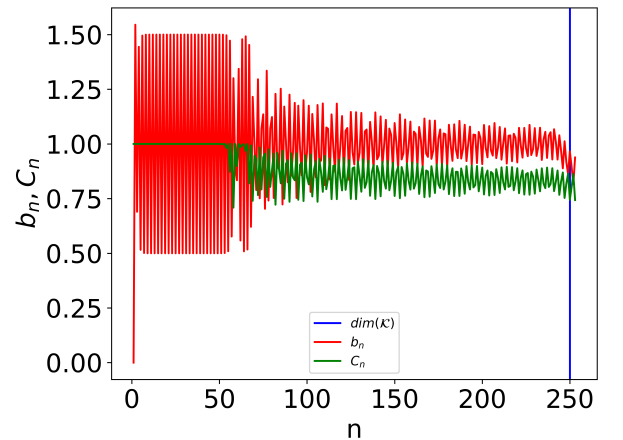
Figure 5. Lanczos sequence b_n and overlap C_n for the one-magnon space of the Heisenberg delta chain with the starting vector |A\rangle . The blue line is drawn at the analytically known dimension of the Krylov space \dim(\mathcal{K}) = 250 .
