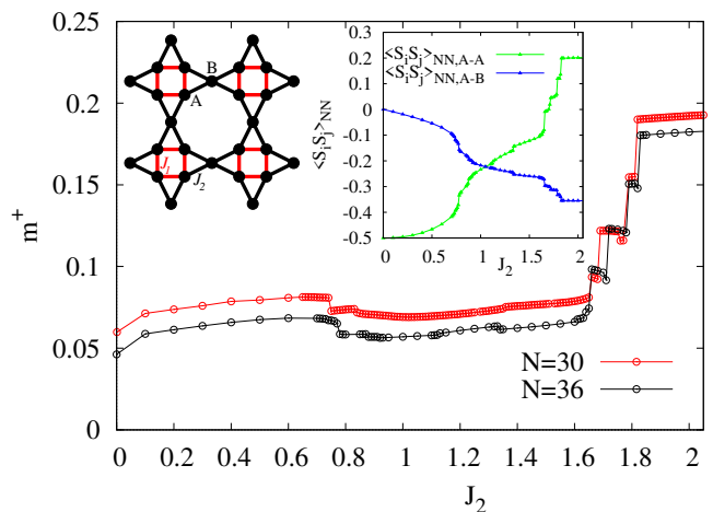
Figure 1. Main panel: Order parameter m^+ as defined in Eq. (3) of the spin-1/2 J_1 - J_2 SKHAF ( N = 30 and 36 ) as a function of J_2 . Left inset: Sketch of the square-kagome lattice. Here A and B label the two non-equivalent sites and J_1 and J_2 label the two non-equivalent nearest-neighbor bonds. Right inset: Nearest-neighbor spin-spin correlation for N = 36 : \langle \mathbf{s}_i \mathbf{s}_j \rangle_{NN,A-A} = (\langle \mathbf{s}_0 \mathbf{s}_1 \rangle + \langle \mathbf{s}_0 \mathbf{s}_3 \rangle)/2 and \langle \mathbf{s}_i \mathbf{s}_j \rangle_{NN,A-B} = (\langle \mathbf{s}_0 \mathbf{s}_4 \rangle + \langle \mathbf{s}_1 \mathbf{s}_4 \rangle)/2 , see Fig. 13 for the numbering of sites.
