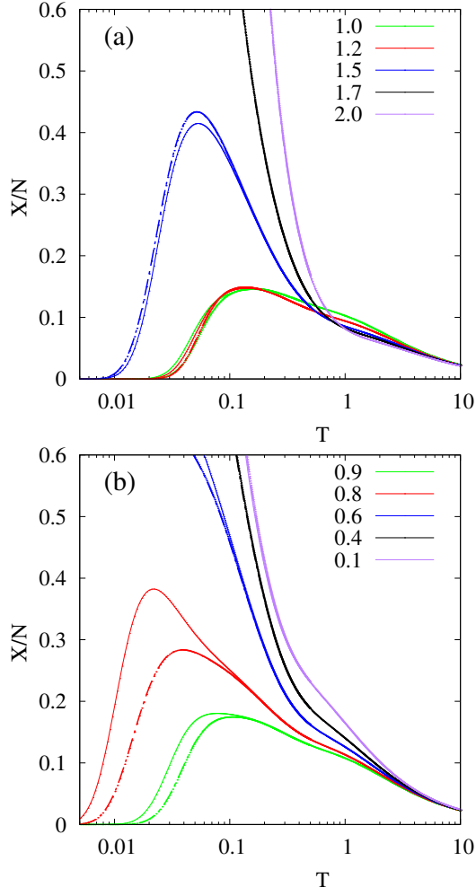
Figure 17. Susceptibility per site X/N for N = 30 (dashed lines) and N = 36 (solid lines). (a) J_2 \geq 1.0 , (b) J_2 \leq 1.0 . Note that in a wide temperature range the corresponding curves for N = 30 and 36 coincide, however, there is a noticeable difference at low T for J_2 \geq 0.8 , see also Fig. 7 in Sec. III B.
