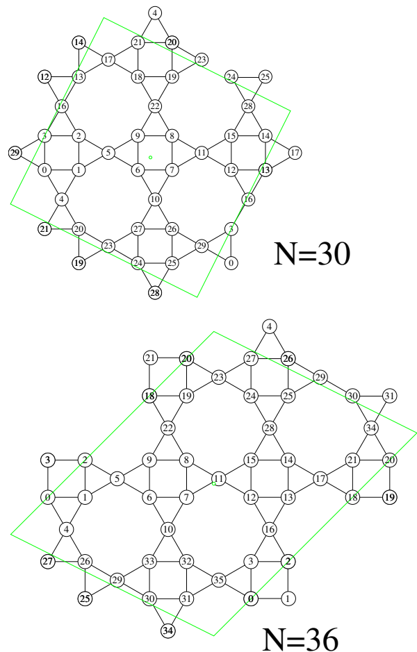
Figure 13. Finite square-kagome lattices of N = 30 and N = 36 sites.
