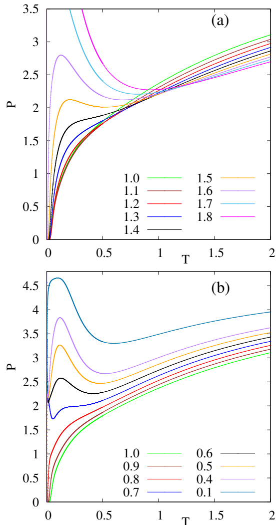
Figure 3. Modified Wilson ratio P(T) , cf. Eq. (4), of the spin-1/2 J_1 - J_2 SKHAF ( N = 36 ). (a) J_2 \geq 1.0 , (b) J_2 \leq 1.0 .
