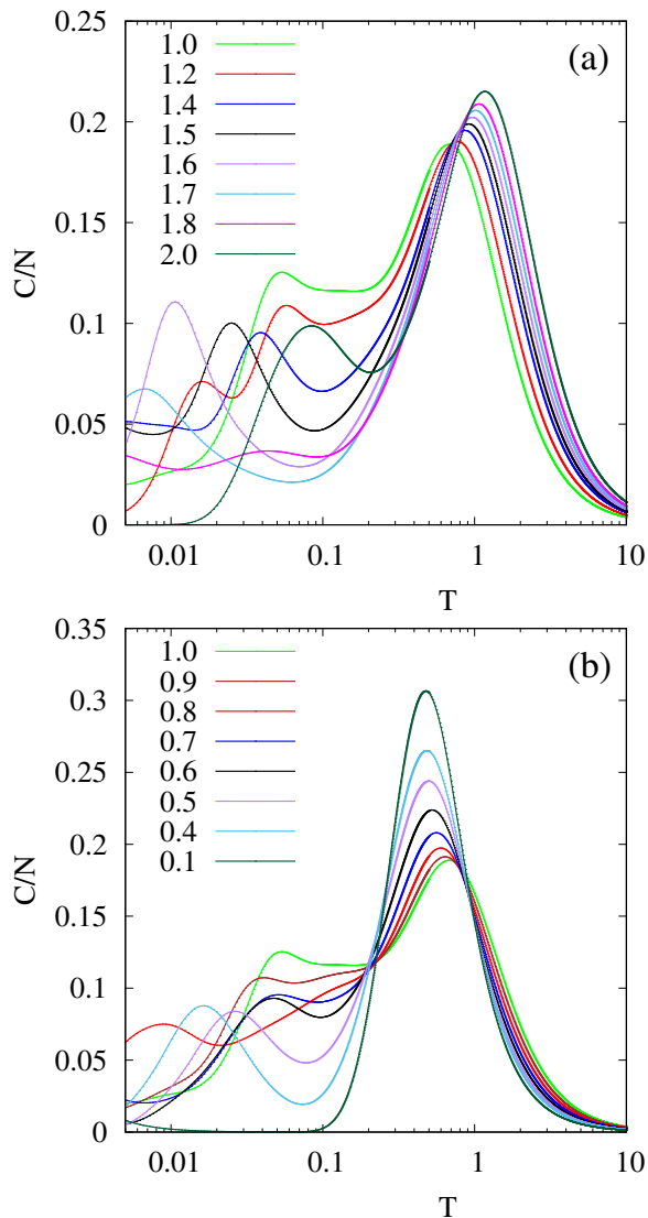
Figure 4. Specific heat C/N of the spin-1/2 J_1 - J_2 SKHAF for N = 36 . (a) J_2 \geq 1.0 , (b) J_2 \leq 1.0 .
