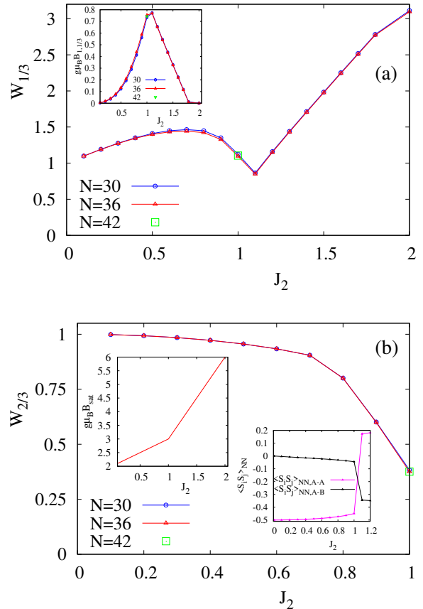
Figure 10. (a) Main panel: Width W_{1/3} = g\mu_B(B_{2,1/3} - B_{1,1/3}) of the 1/3 plateau of the J_1 - J_2 SKHAF for N = 30 and 36 . For J_2 = 1 data for N = 42 [29] are added. Inset: Lower edge g\mu_B B_{1,1/3} of the 1/3 plateau as a function of J_2 for N = 30 and 36 . (b) Width W_{2/3} = g\mu_B(B_{2,2/3} - B_{1,2/3}) of the 2/3 plateau of the SKHAF for N = 30 and 36 . For J_2 = 1 data for N = 42 [29] are added. Left inset: Saturation field g\mu_B B_{\text{sat}} as a function of J_2 . Right inset: Nearest-nearest correlation functions \langle \mathbf{s}_i \mathbf{s}_j \rangle_{NN,A-A} and \langle \mathbf{s}_i \mathbf{s}_j \rangle_{NN,A-B} in the 1/3 plateau state.
