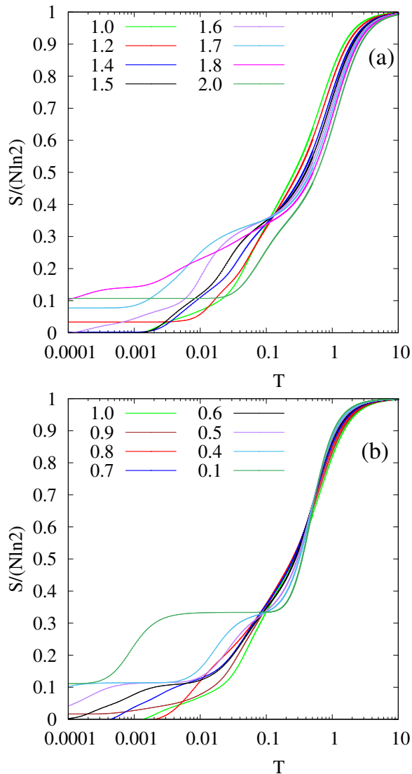
Figure 6. Entropy S/N of the spin-1/2 J_1 - J_2 SKHAF for N = 36 . (a) J_2 \geq 1.0 , (b) J_2 \leq 1.0 . Note that the finite entropy at T = 0 for J_2 = 1.8 and 2.0 is caused by the ferrimagnetic multiplet and by an accidental degeneracy of the ground state for some other values of J_2 .
