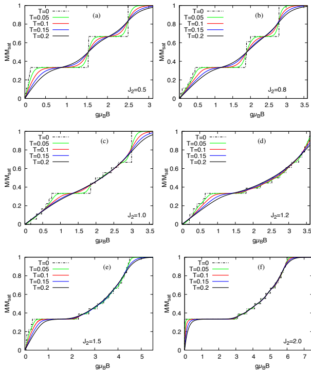
Figure 11. Finite temperature magnetization curves M(T, B) of the J_1 - J_2 SKHAF with N = 36 sites for selected values of J_2 .
