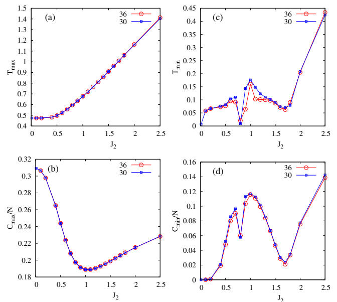
Figure 5. Features of the main maximum and the minimum below the main maximum in the temperature profile of the specific heat C(T)/N of the spin-1/2 J_1 - J_2 SKHAF ( N = 30 and N = 36 ). (a) Position T_{\max} and (b) height C_{\max}/N of the main maximum. (c) Position T_{\min} and (d) depth C_{\min}/N of the minimum.
