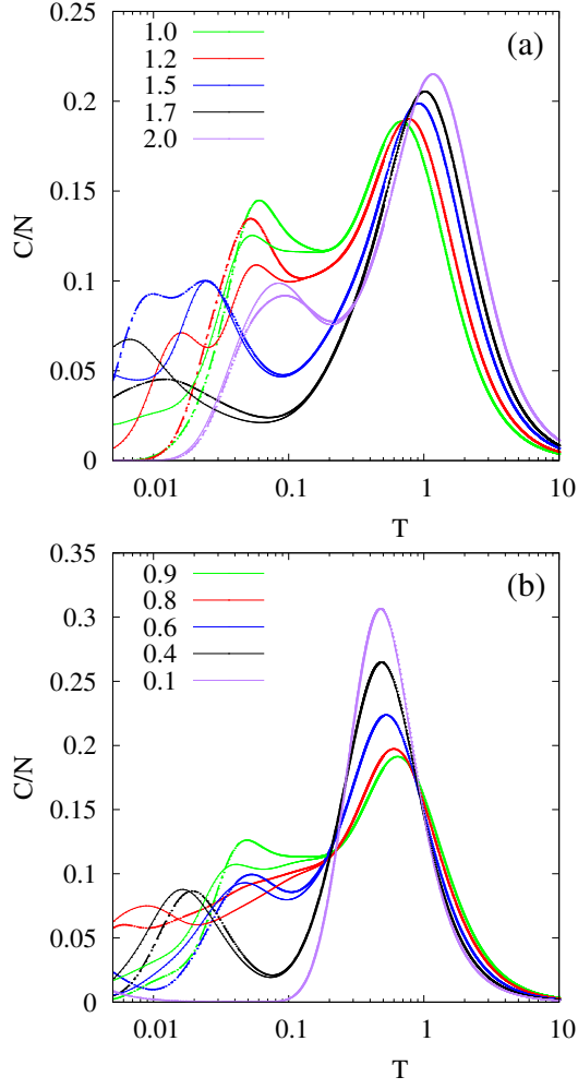
Figure 15. Specific heat per site C/N for N = 30 (dashed lines) and N = 36 (solid lines). (a) J_2 \geq 1.0 , (b) J_2 \leq 1.0 . Note that in a wide temperature range the corresponding curves for N = 30 and 36 coincide.
