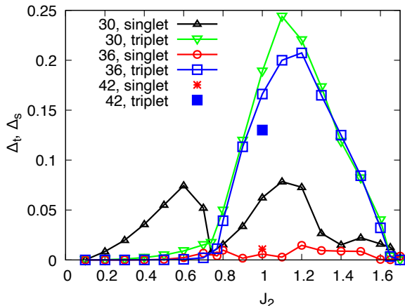
Figure 2. Singlet-triplet and singlet-singlet gaps \Delta_t and \Delta_s of the spin-1/2 J_1 - J_2 SKHAF ( N = 30 and 36 ) as a function of J_2 . For J_2 = 1 data for N = 42 [29] are added.
