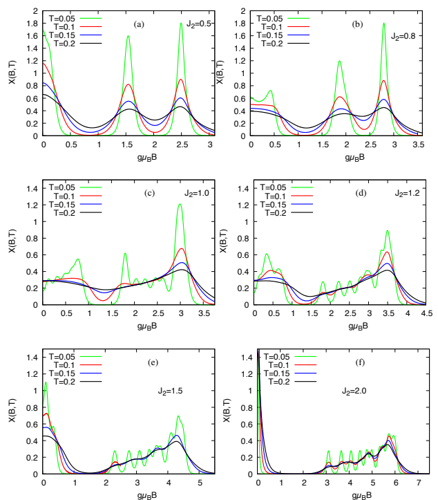
Figure 12. Differential susceptibility X(T, B) = dM(T, B)/d(g\mu_B B) of the J_1 - J_2 SKHAF with N = 36 sites for selected values of J_2 .
