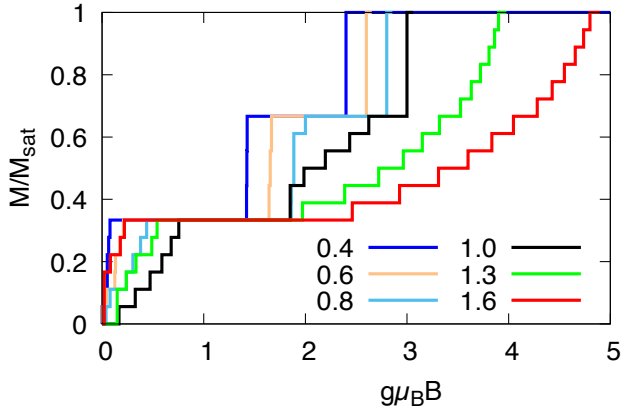
Figure 9. Zero-temperature magnetization curve of the J_1 - J_2 SKHAF with N = 36 sites and selected values of J_2 .
