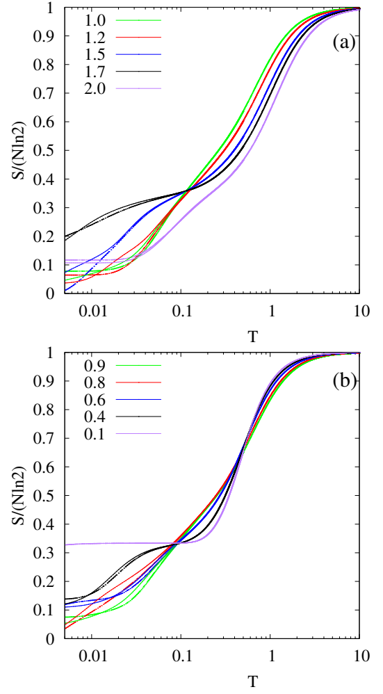
Figure 16. Entropy per site S/N for N = 30 (dashed lines) and N = 36 (solid lines). (a) J_2 \geq 1.0 , (b) J_2 \leq 1.0 . Note that in a wide temperature range the corresponding curves for N = 30 and 36 coincide.
