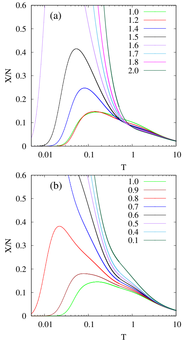
Figure 7. Susceptibility X/N of the spin-1/2 J_1 - J_2 SKHAF for N = 36 . (a) J_2 \geq 1.0 , (b) J_2 \leq 1.0 .
