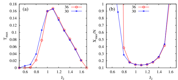
Figure 8. Features of the maximum in the temperature profile of the susceptibility X(T)/N of the spin-1/2 J_1 - J_2 SKHAF ( N = 30 and N = 36 ). (a) Position T_{\max} of the maximum. (b) Height X_{\max}/N of the maximum.
