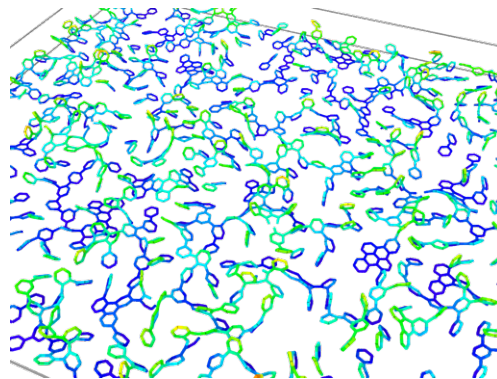
Figure 11. A typical result of vertical momentum dynamics with missing molecules applied to BPT-SAM after 4900 time steps, T = 300 \text{ K} , k = 60 \frac{\text{eV}}{\text{\AA}} . Color represents position along z -direction (blue to red as on regular maps). x - and y -directions as in Fig. 4.
