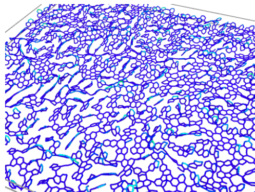
Figure 7. A typical result of vertical momentum dynamics applied to NPTH-SAM, T = 700 K, k = 30 \frac{\text{eV}}{\text{\AA}} . Color represents position along z -direction (blue to red as on regular maps). x - and y -directions as in Fig. 4.
