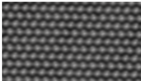
Figure 15. Simulated atomic force microscopy image of a TPT-based self-assembled monolayer.
