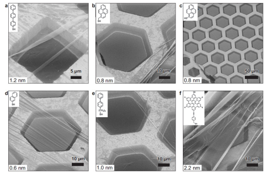
Figure 1. Macroscopic CNMs made from various precursors resting on support structures. Images, made using helium ion microscopy, are taken from [8] (with friendly permission).
