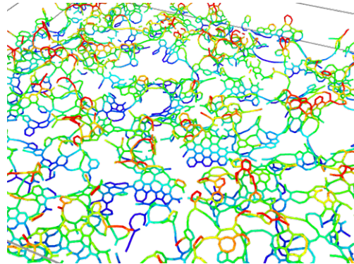
Figure 8. A typical result of vertical and lateral momentum dynamics applied to BPT-SAM after 4900 time steps, T = 300 \text{ K} , v = 35 \frac{\text{\AA}}{\text{ps}} , k = 60 \frac{\text{eV}}{\text{\AA}} . Color represents position along z -direction (blue to red as on regular maps). x - and y -directions as in Fig. 4.
