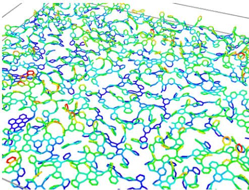
Figure 5. A typical result of vertical momentum dynamics applied to BPT-SAM, T = 700 K, k = 60 \frac{\text{eV}}{\text{\AA}} . Color represents position along z -direction (blue to red as on regular maps). x - and y -directions as in Fig. 4.
