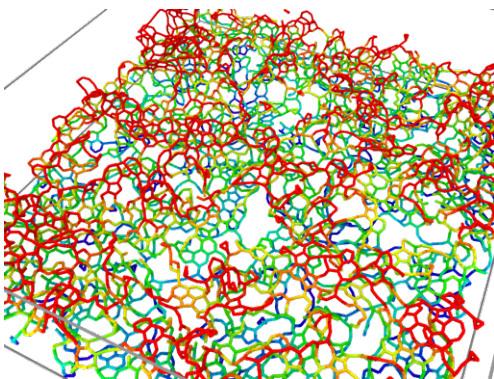
Figure 10. A typical result of vertical and lateral momentum dynamics applied to TPT-SAM after 5700 time steps, T = 700 \text{ K} , v = 35 \frac{\text{\AA}}{\text{ps}} , k = 30 \frac{\text{eV}}{\text{\AA}} . Color represents position along z -direction (blue to red as on regular maps). x - and y -directions as in Fig. 4.
