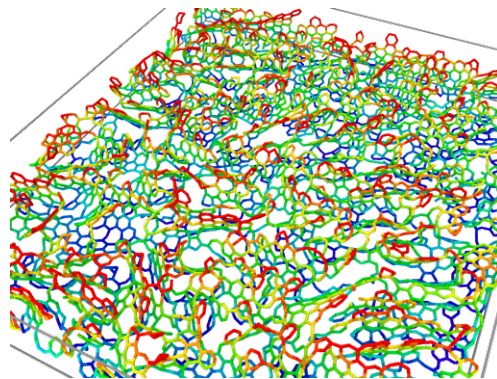
Figure 6. A typical result of vertical momentum dynamics applied to TPT-SAM, T = 700 K, k = 30 \frac{\text{eV}}{\text{\AA}} . Color represents position along z -direction (blue to red as on regular maps). x - and y -directions as in Fig. 4.
