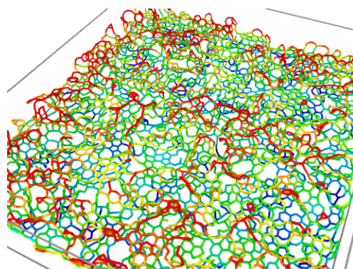
Figure 12. A typical result of vertical momentum dynamics with missing molecules applied to TPT-SAM after 7200 time steps, T = 300 \text{ K} , k = 60 \frac{\text{eV}}{\text{\AA}} . Color represents position along z -direction (blue to red as on regular maps). x - and y -directions as in Fig. 4.
