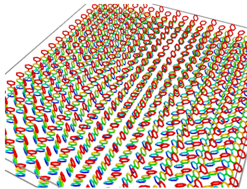
Figure 4. A typical result of minimization of a weakly randomized TPT-based CNM. Color represents position along z -direction (blue to red as on regular maps). The x -coordinate runs along the visible rows from bottom to top and the y -coordinate perpendicular to that, i.e. from left to right.
