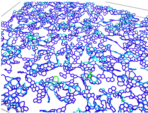
Figure 9. A typical result of vertical and lateral momentum dynamics applied to NPTH-SAM after 2500 time steps, T = 300 \text{ K} , v = 35 \frac{\text{\AA}}{\text{ps}} , k = 60 \frac{\text{eV}}{\text{\AA}} . Color represents position along z -direction (blue to red as on regular maps). x - and y -directions as in Fig. 4.
