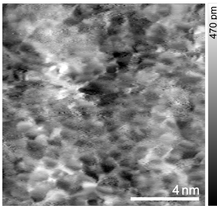
Figure 2. AFM tapping mode topography image of TPT CNM on Au, measured at 93 K in ultra-high vacuum (amplitude set point A = 7.6 nm, center frequency f_0 = 274.8 kHz). The height information is black-to-white encoded, displaying the subnanoporous network of the nanomembrane.
