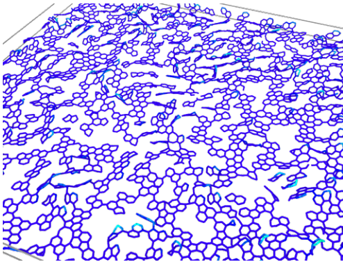
Figure 13. A typical result of vertical momentum dynamics with missing molecules applied to NPTH-SAM after 2500 time steps, T = 300 K, k = 60 \frac{\text{eV}}{\text{\AA}} . Color represents position along z -direction (blue to red as on regular maps). x - and y -directions as in Fig. 4 .
