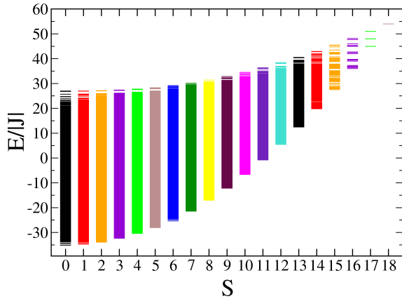
FIG. 2: (Color online) Complete energy spectrum of the antiferromagnetic cuboctahedron with s = 3/2 .
