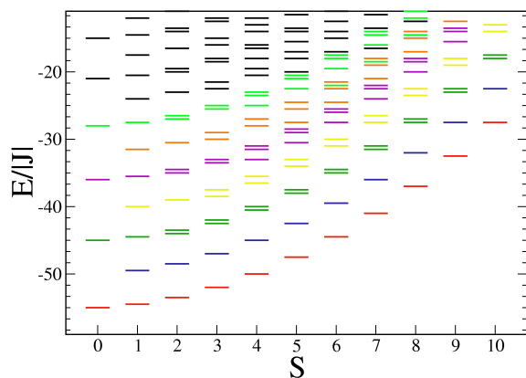
FIG. 6: (Color online) Part of the energy spectra of the rotational-band Hamiltonian for an antiferromagnetic spin ring N = 8 , s = 5/2 . Seven super-bands are colored.
