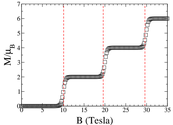
FIG. 10: (Color online) Approximate spectrum of a spin ring with N = 12 spins s = 5/2 calculated using 8 bands, D_2 point-group symmetry and the approximate selection rule in Eq. (24) (top). Corresponding magnetization of the system (bottom). The dashed red lines refer to experimental data of the first three magnetization steps from Ref. 40 with J = 35.2 K and k_B T/J = 0.01 .
