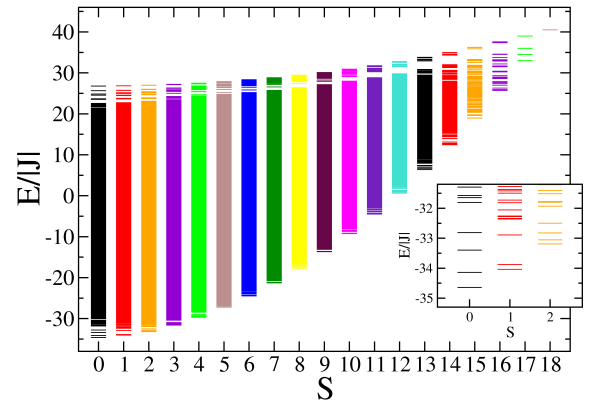
FIG. 4: (Color online) Complete energy spectrum of the antiferromagnetic truncated tetrahedron with J_1 = J_2 = J . The inset shows low-lying levels in subspaces with S = 0, 1, 2 .
