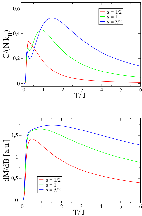
FIG. 5: (Color online) Specific heat c(T, B = 0) (top) and differential magnetic susceptibility \chi(T, B = 0) (bottom) of the truncated tetrahedron with J_1 = J_2 = J .
