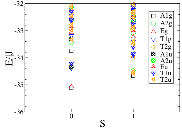
FIG. 3: (Color online) Low-lying energy spectrum of the antiferromagnetic cuboctahedron with s = 3/2 in subspaces of S = 0 and S = 1 . The symbols denote the irreducible representations of the O_h group.
