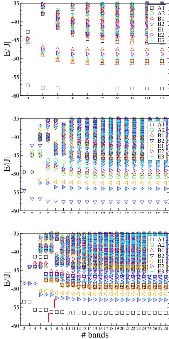
FIG. 7: (Color online) Energy levels of an antiferromagnetic spin ring N = 8 with s = 5/2 as a function of the number of occupied rotational-bands used for diagonalization in subspaces S = 0 (top), S = 1 (center) and S = 2 (bottom). The arrows in the S = 2 subspace refer to the steps within the convergence behavior mentioned in the text. The states are labeled according to irreducible representations of D_8 .
