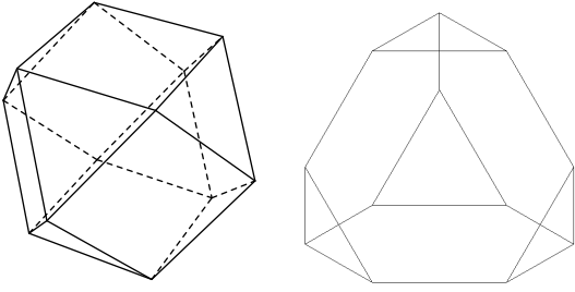
FIG. 1: Structure of the cuboctahedron (l.h.s.) and the truncated tetrahedron (r.h.s.). 27
