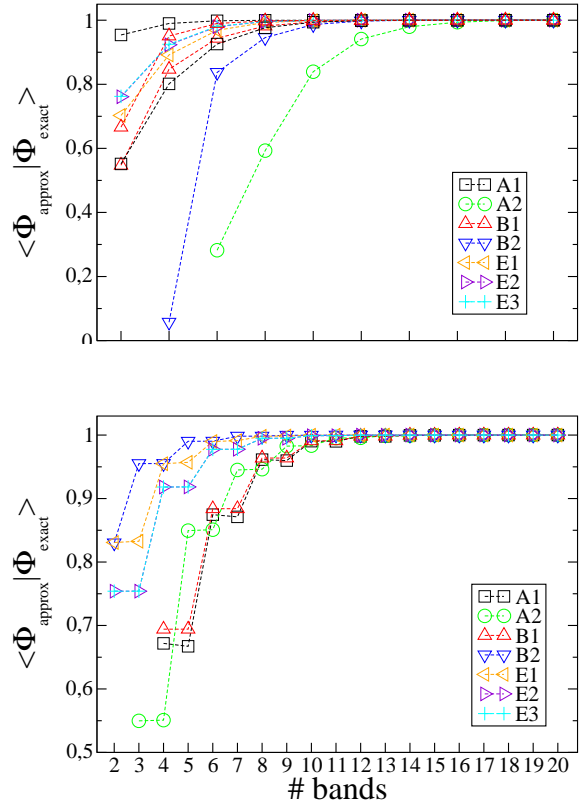
FIG. 8: (Color online) Convergence of the eigenstates of an antiferromagnetic spin ring N = 8 with s = 5/2 as a function of the number of occupied rotational-bands used for diagonalization in subspaces S = 0 (top) and S = 1 (bottom). The states are labeled according to irreducible representations of D_8 .
