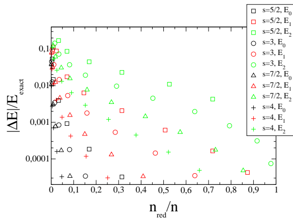
FIG. 9: (Color online) Relative difference between approximate and exact energy eigenvalues for the lowest states of the first three occupied rotational-bands for an antiferromagnetic spin ring N = 8 with various s and total spin S = 0 . E_0 refers to the energy of the lowest state of the first rotational-band, E_1 to the lowest state of the second rotational-band and E_2 to the lowest state of the third rotational-band respectively.
