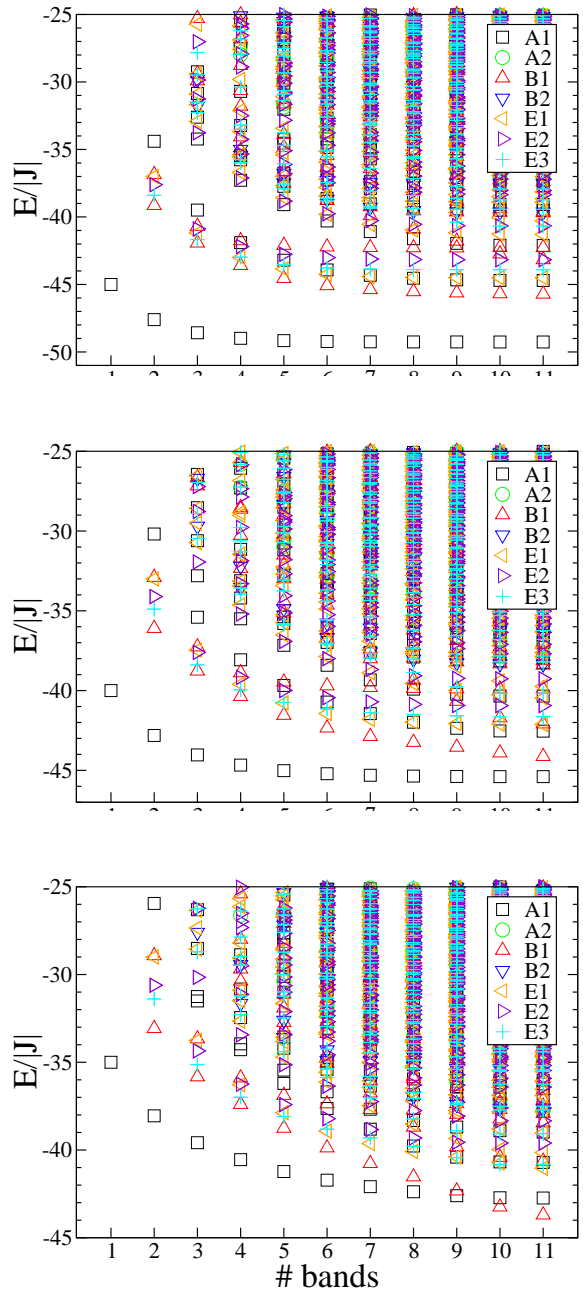
FIG. 11: (Color online) Energy levels of an antiferromagnetic spin ring N = 8 with s = 5/2 and additional next-nearest-neighbor coupling J_{nnn} as a function of the number of occupied rotational-bands used for diagonalization in subspaces S = 0 with J_{nnn}/J_{nn} = 0.2 (top), J_{nnn}/J_{nn} = 0.3 (center) and J_{nnn}/J_{nn} = 0.4 (bottom). The states are labeled according to irreducible representations of D_8 .
