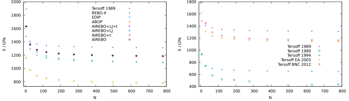
Figure 1: Young’s modulus of graphene for various sizes and potentials.
