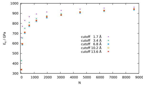
Figure 5: Young’s modulus of diamond taken along the x -direction shown in Fig. 4 for the AIREBO+LJ potential with various cutoffs.
