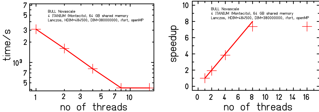
Fig. 1. Scaling of CPU time for 200 Lanczos iterations with number of allowed threads. The machine has eight cores.
