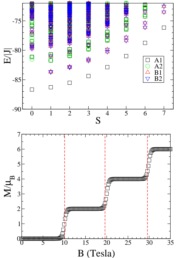
FIG. 10: (Color online) Approximate spectrum of a spin ring with N = 12 spins s = 5/2 calculated using 8 bands, D_2 point-group symmetry and the approximate selection rule in Eq. (24) (top). Corresponding magnetization of the system (bottom). The dashed red lines refer to experimental data of the first three magnetization steps from Ref. 40 with J = 35.2 K and k_B T/J = 0.01 .
