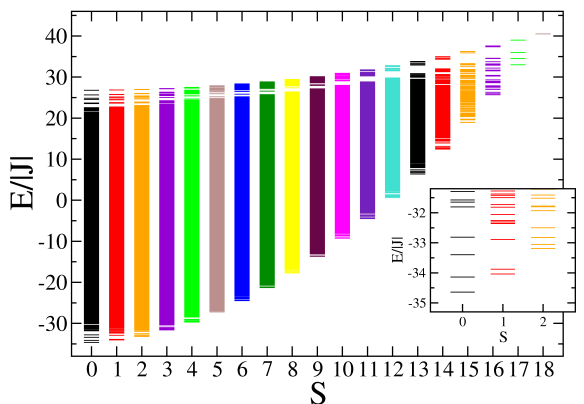
FIG. 4: (Color online) Complete energy spectrum of the antiferromagnetic truncated tetrahedron with J_1 = J_2 = J . The inset shows low-lying levels in subspaces with S = 0, 1, 2 .
