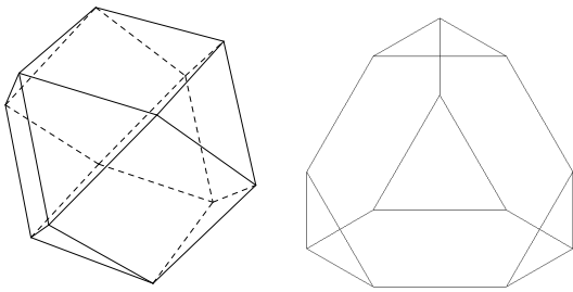
FIG. 1: Structure of the cuboctahedron (l.h.s.) and the truncated tetrahedron (r.h.s.). 27
